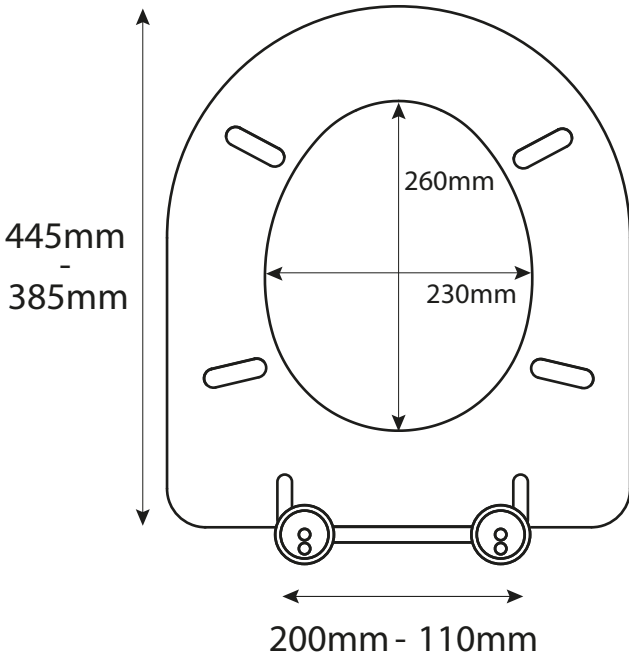
Max/Min Adjustment
